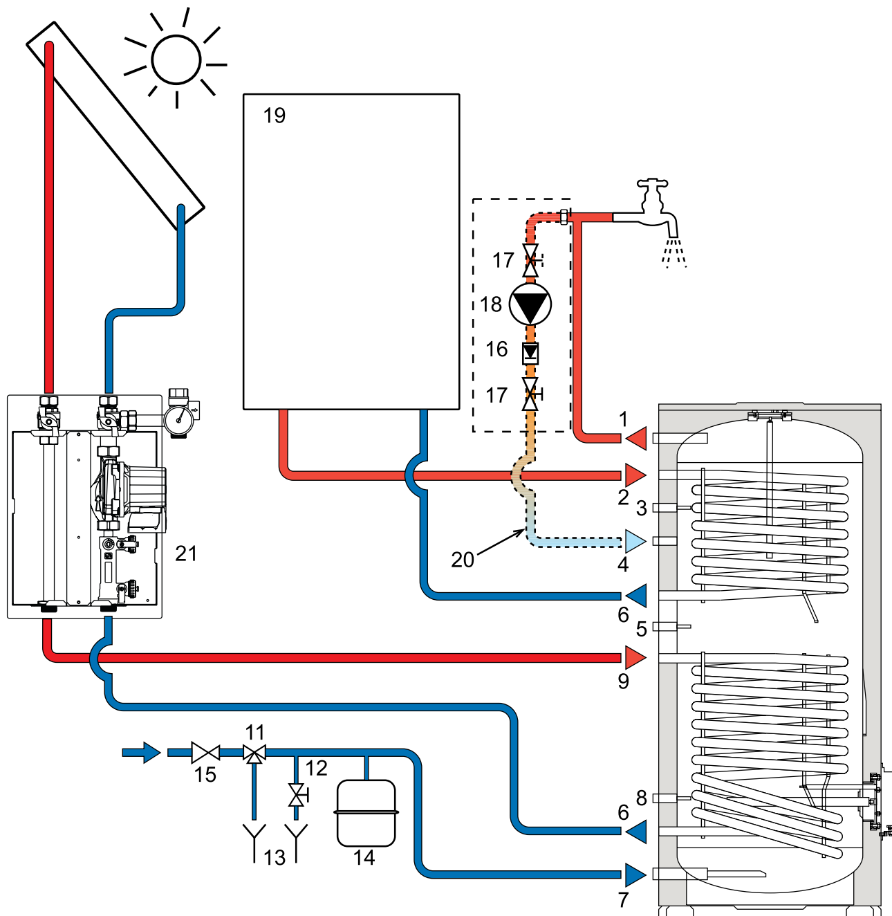
fig.6 - Circuit Hidraulic ECUNIT F 2C
